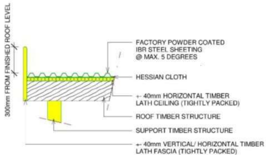
RVHOA - STEEL ROOF SHEETING MINIMUM REQUIREMENTS
